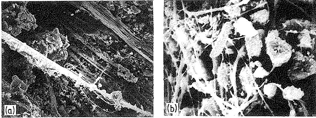
Figure 8 (a) Chrysotile fibrils remaining in a cement trough after pull-out. At higher magnification (b) the complex interaction between these fibrils and the cement particles is clearly illustrated.
