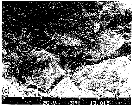
Figure 1 Calcium silicate hydrate of the needle morphology which interlocks and binds cement particles together, (a) and (b), as well as microcracks formed during curing (c).
