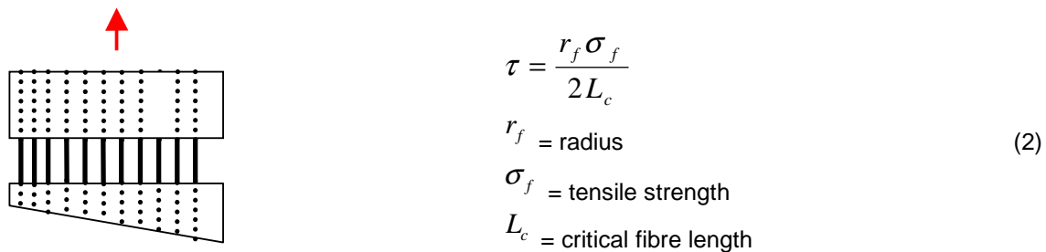
Fig. 7 Fibre pull-out test arrangement for the determination of critical fibre length
