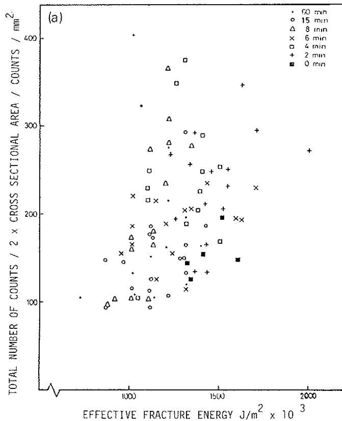
Figure 5 (a) Plot of total number of acoustic emission counts with corresponding fracture energy for a range of fiberising times (i.e. asbestos fibre bundle separation procedure) (b) Approximate relationship between cumulative integral of acoustic emission and effective fracture energy. (Line drawn by simple regression analysis)
