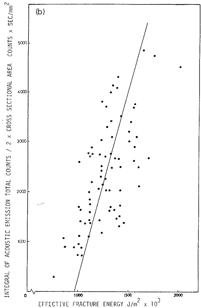
Figure 5 (a) Plot of total number of acoustic emission counts with corresponding fracture energy for a range of fiberising times (i.e. asbestos fibre bundle separation procedure) (b) Approximate relationship between cumulative integral of acoustic emission and effective fracture energy. (Line drawn by simple regression analysis)
